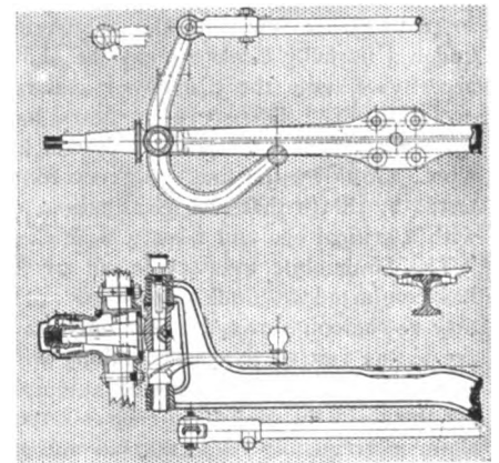
Timken Front Axle.
